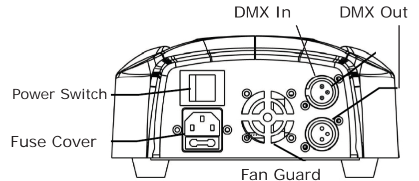
Figure 2: The Rear Connections
